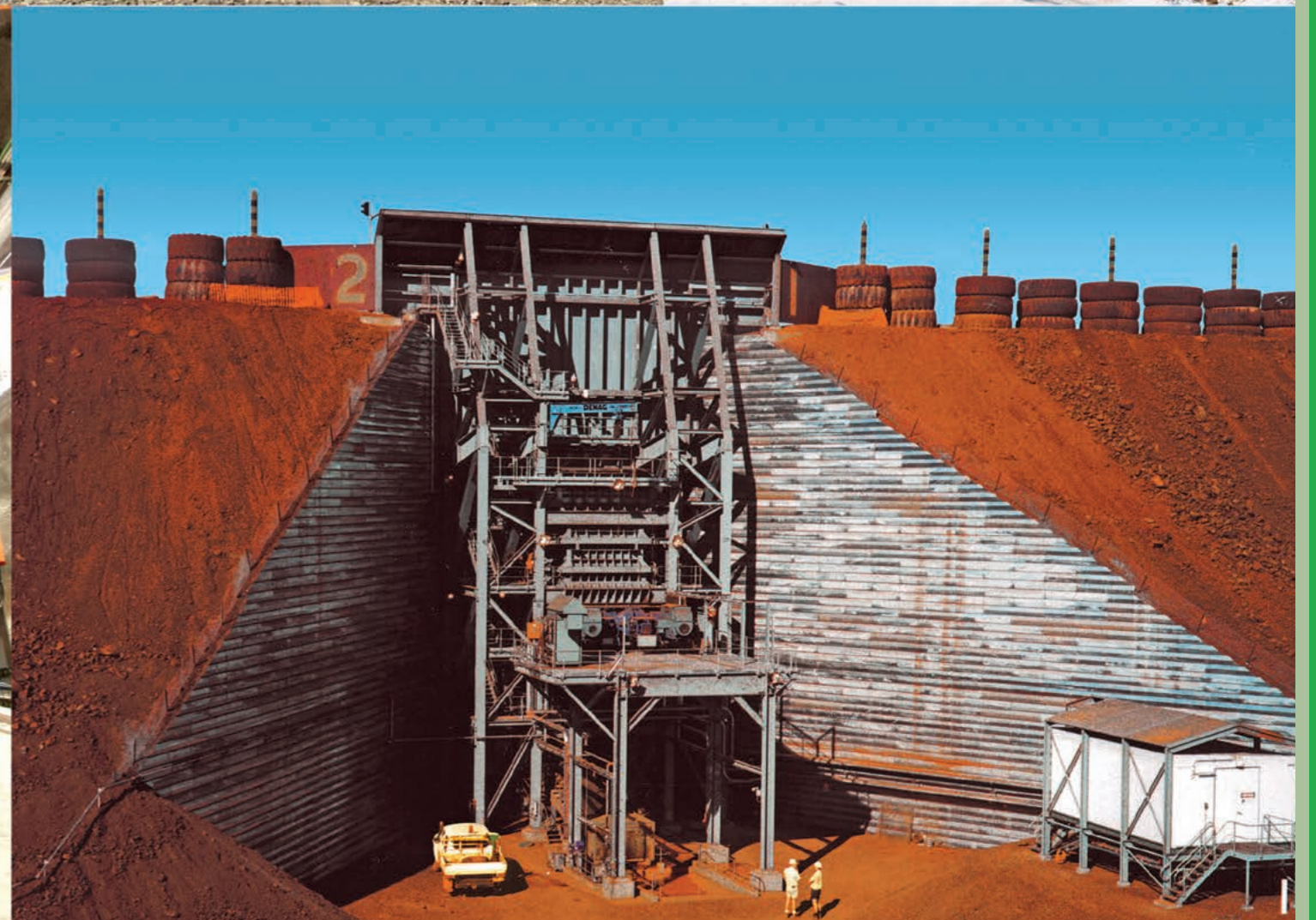
Iron Ore | Australia | In: 2,500mm | Out: -250mm | Capacity: 6,000TPH
