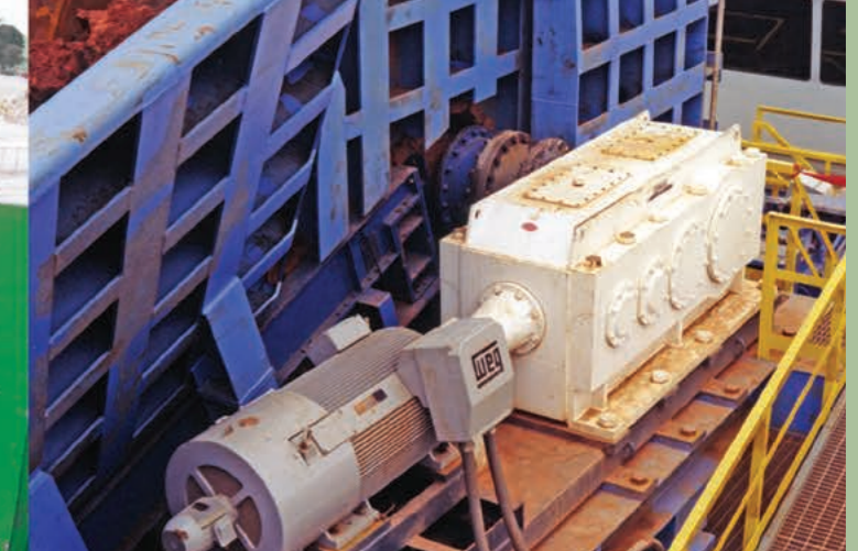
D7 Apron Plate Feeder with electro-mechanical drive
