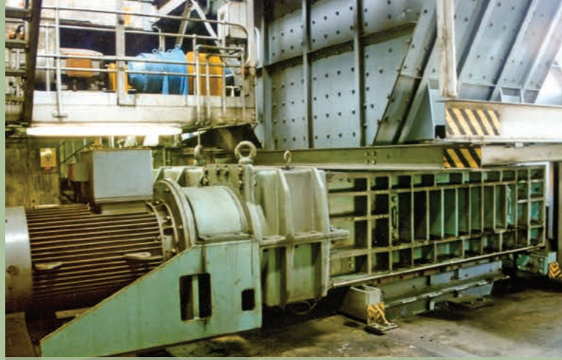
Coal | South Africa | In: 1,000mm | Out: -180mm | Capacity: 900TPH
