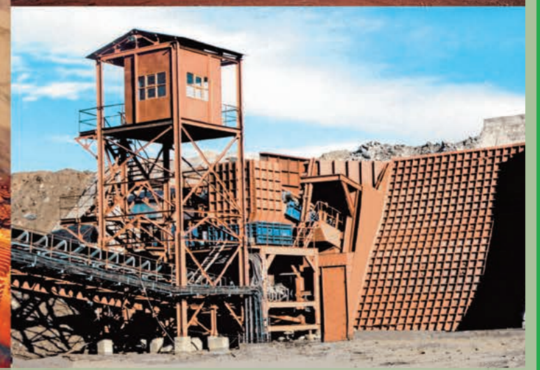
Limestone | India | In: 300mm | Out: -150mm | Capacity: 700TPH
