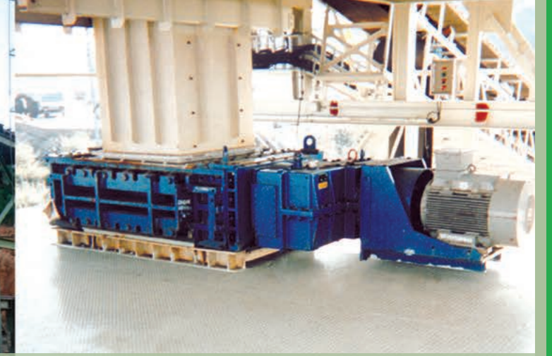
Lignite | Spain | In: 180mm | Out: -30mm | Capacity: 10TPH
