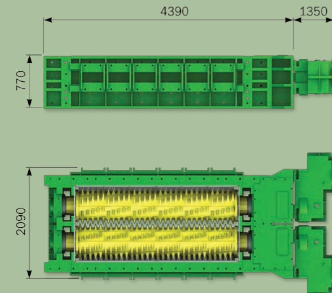
All dimensions are in millimetres, and may vary dependant upon configuration
