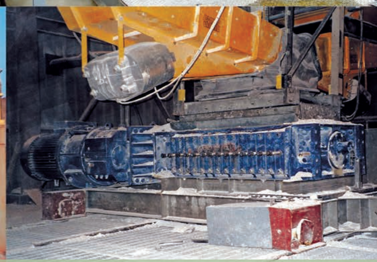
Burnt Lime | UK | In: 125mm | Out: -40mm | Capacity: 100TPH
