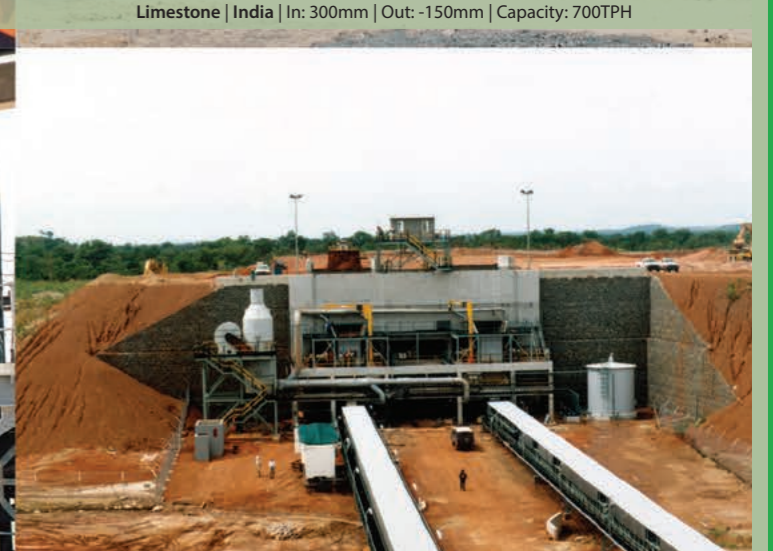
Lateritic Gold Ore/Clay | Mali | In: 1,000mm | Out: -250mm | Capacity: 750TPH
